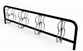
RF7620AM Urban A Double Sided Bicycle Rack L x W x H: 2080 mm x 400 mm x 550 mm Underground concrete foundation.
